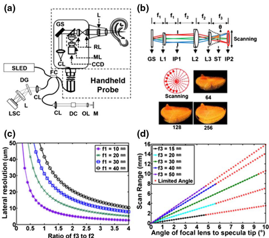
Fig. 1. (a) Schematic diagram of the spectral domain (SD)-OCT system. (b) Schematic of the OCT probe based on a relay lens and 3D reconstructions according to sampling numbers (64, 128, 256). (c) Simulated lateral resolutions for the OCT as a ratio of the focal length of Lens 3 ( f_3 ) to the focal length of Lens 2 ( f_2 ); each colored line shows the value of the focal length of Lens 1 ( f_1 ). (d) Simulated scanning range according to the scanning angle ( \theta ) from the center of Lens 3 to the edge of the specula tip for different f_3 . The red lines indicate a limited angle. Abbreviations: CL, collimator; DC, dispersion compensation unit (hardware-based dispersion compensation unit was connected to the reference arm path to compensate the dispersion); DG, diffraction grating; FC, fiber coupler; GS, galvanometer scanners; L, lens; LSC, line-scanning camera; ML, magnifier lens; M, mirror; OL, objective lens, CCD, charge-coupled device, FL, focal length, PC, polarization controllers; RL, relay lens; ST, specula tip; SLED, superluminescent diode.
